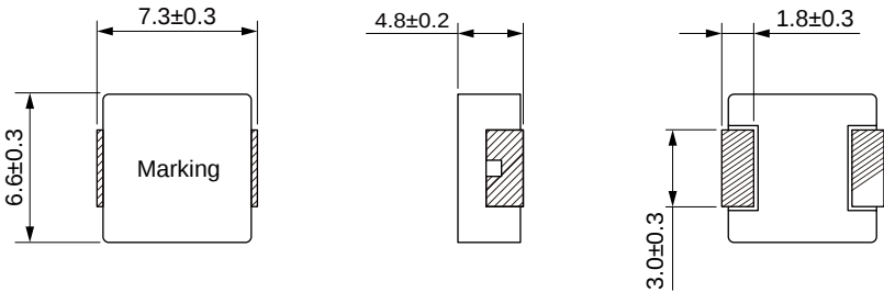
Dimensions: [mm]
