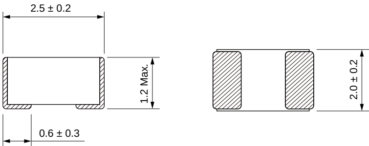
Dimensions: [mm]
