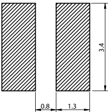
Land Pattern: [mm]
